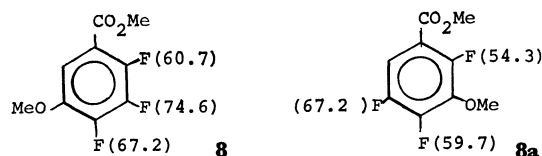
Fig. 1. Calculated 19 F NMR chemical shift for 8 and 8a .
